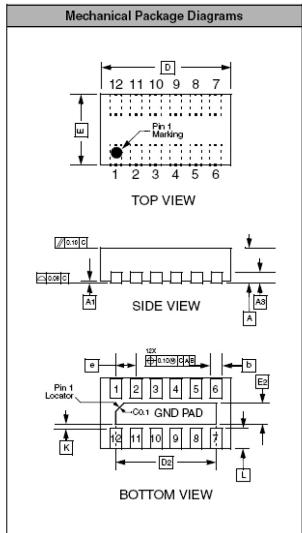
Dimensions for 12-Lead, 0.4mm pitch µDFN Package
